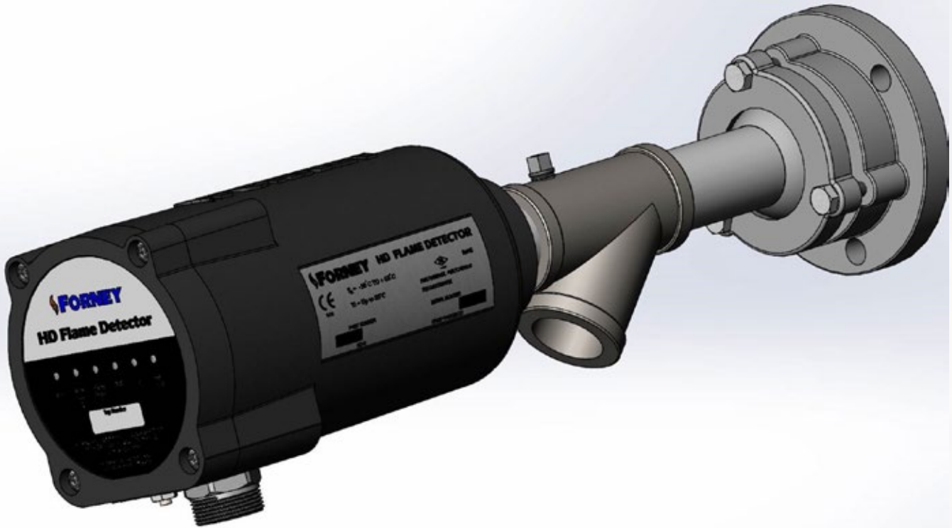
Figure 7 - Swivel Mount, Wye and Detector Assembly
