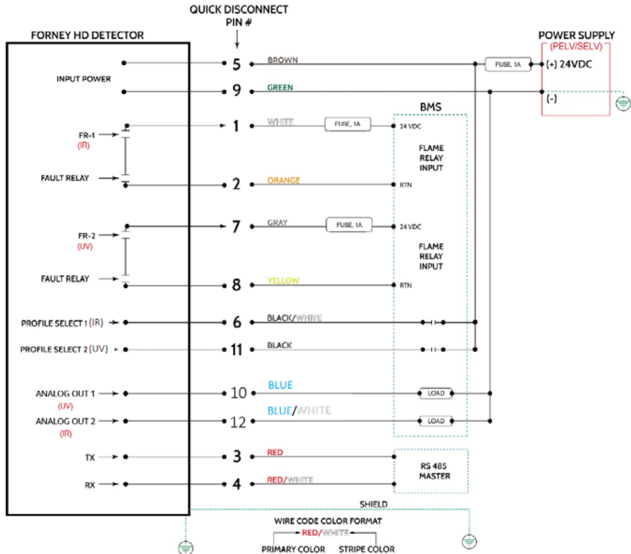
Figure 8 - 12-Pin, Wiring Diagram
